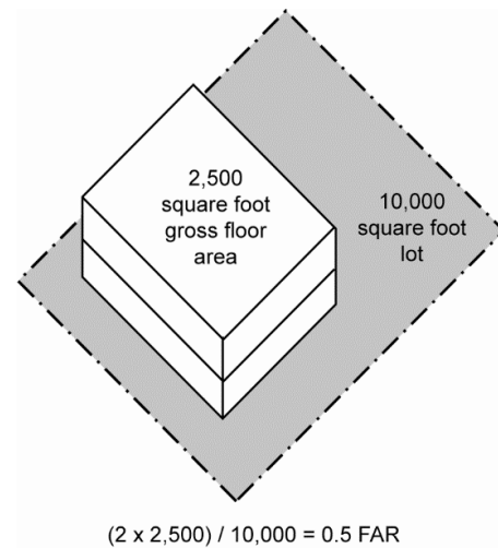
FIGURE 20.24701-1 EXAMPLE OF FLOOR AREA RATIO (FAR)
