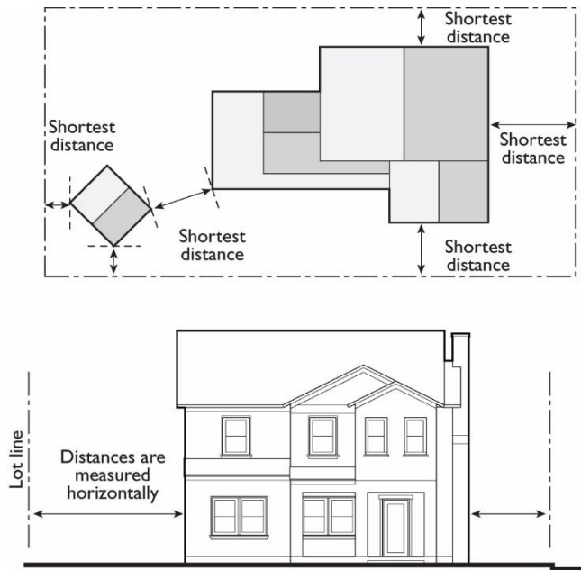
FIGURE 20.103-A: MEASURING DISTANCES
