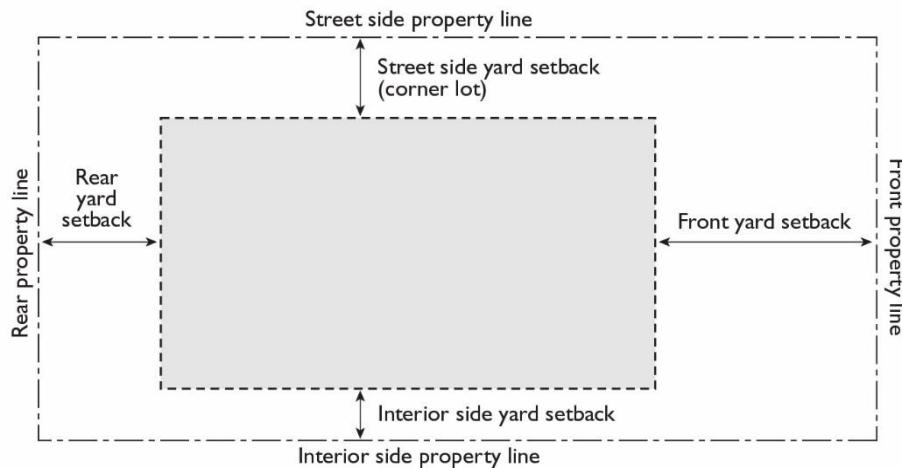
FIGURE 20.103-H: DETERMINING SETBACKS (YARDS)
